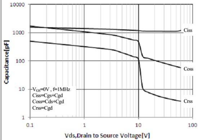
Figure 4. Capacitance Characteristics
