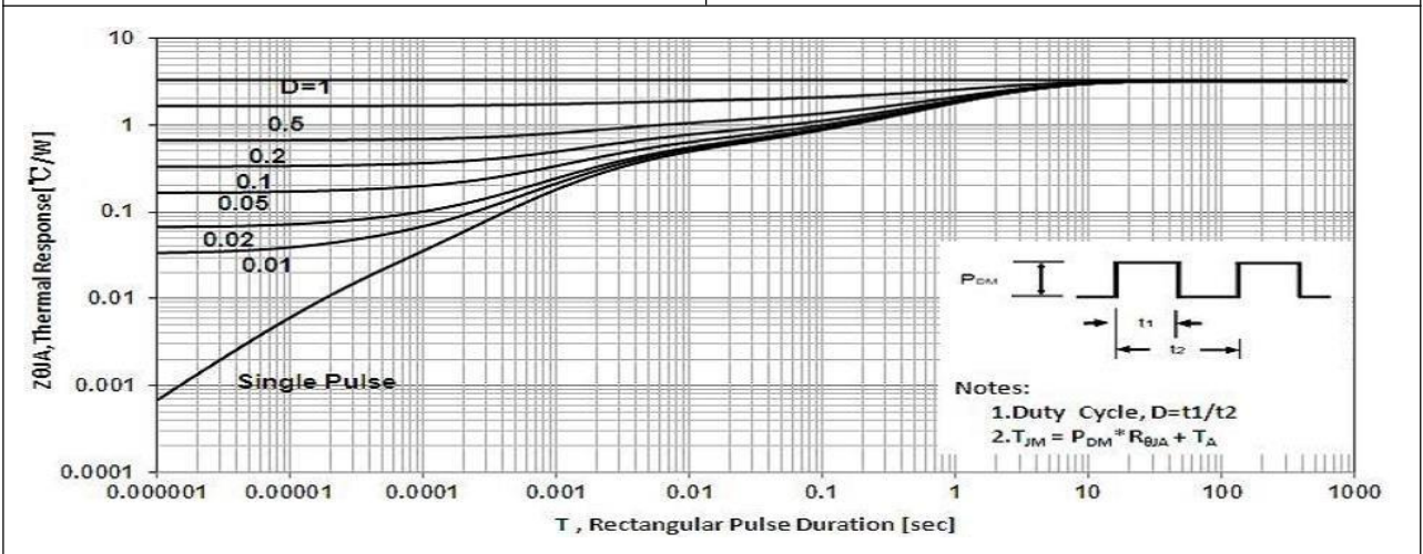
Figure 9. Maximum Effective Thermal Impedance , Junction to Case
